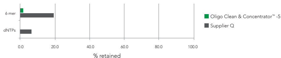
Nucleotide Retention
